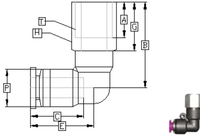
Female Elbow
